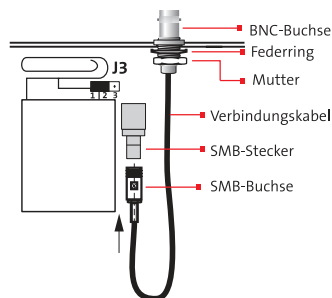
Stabantenne FWA-SA1
